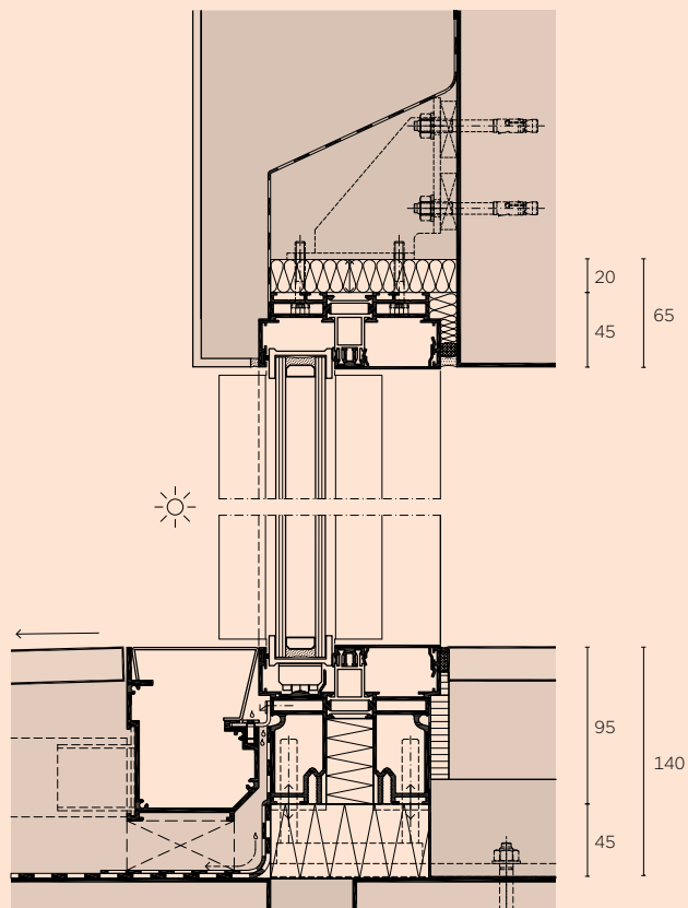
Sockel Original
